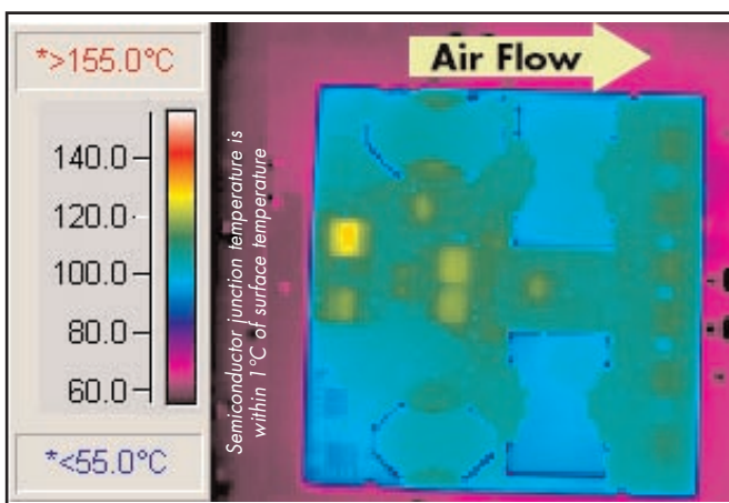
Figure 6: Thermal plot of converter at 23 amp load current with 55°C air flowing at the rate of 200 LFM. Air is flowing across the converter from input to output (nominal input voltage).
